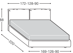
LM50F Base FASCIA
