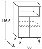
Sideboard with Ecke base Madia con base Ecke
