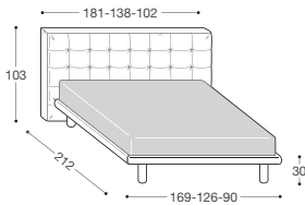
LM12N Base LUNA
