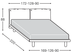
LM50N Base LUNA
