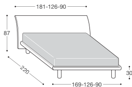
LM1N Base LUNA
