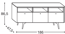
Sideboard with Ecke base Madia con base Ecke
